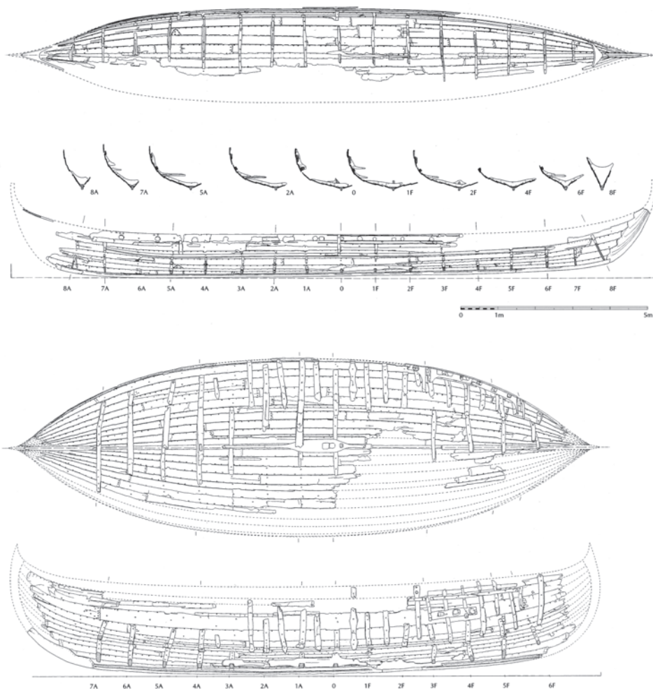
Fig. 7. The diversity of vessels of the Late Viking Age was realised within the Skuldelev finds. Top : Torso drawing of the coastal warship Skuldelev 5. The warship is characterised in general by its extreme aspect ratio varying between 1:7 and 1:9, its very light and flexible construction, the need for a large crew and the large number of oars. Bottom : Torso drawing of the ocean-going vessel Skuldelev 1. This cargo ship is characterised in general by its moderate aspect ratio varying between 1:3 and 1:5, its relatively large, heavy-built construction, its limited number of crew members and few or no oars (Drawing: Sune Villum Nielsen, The Viking Ship Museum).
