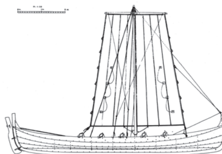
Fig. 1. A Norwegian square-rigged vessel from the 19 th century (Drawing: Bernhard Færøyvik, after Andersen & Andersen 1989).
